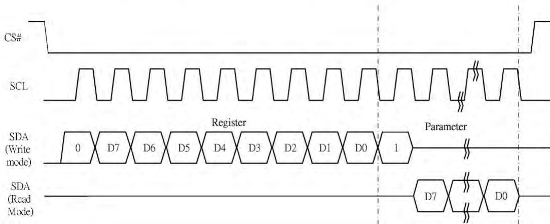
Figure 6-4: Read procedure in 3-wire SPI mode
