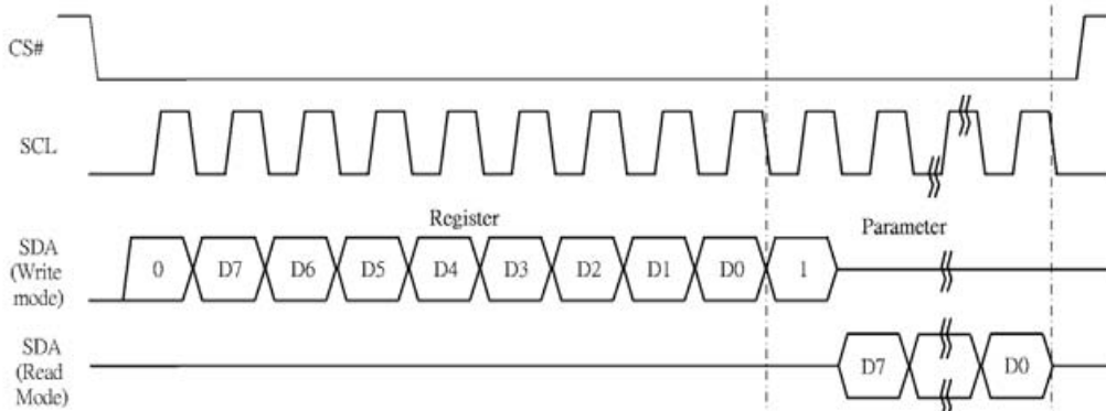
Figure 6-4: Read procedure in 3-wire SPI mode
